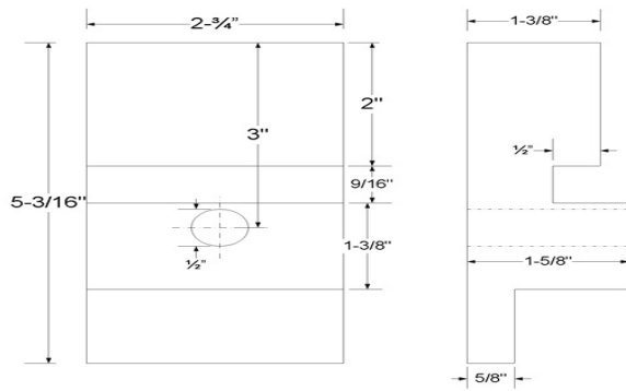
1947 Ford Pickup Rear Cab Mount
